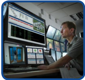
PremiSys™ Software
